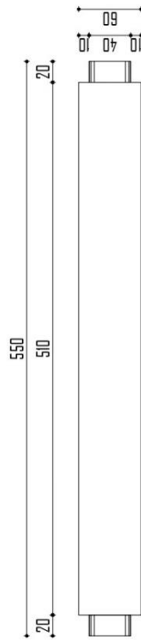
VISTA FRONTAL
