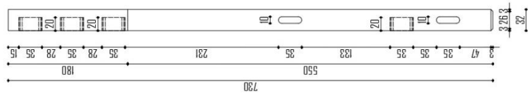
VISTA FRONTAL
