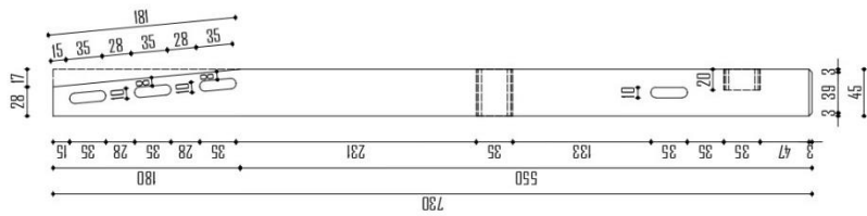
VISTA LATERAL INTERIOR
