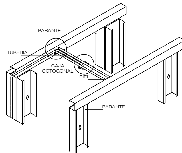
ISOMETRICO INST. ELECT. Esc. S/E
