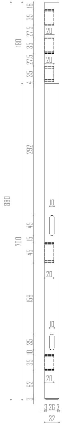
VISTA FRONTAL
