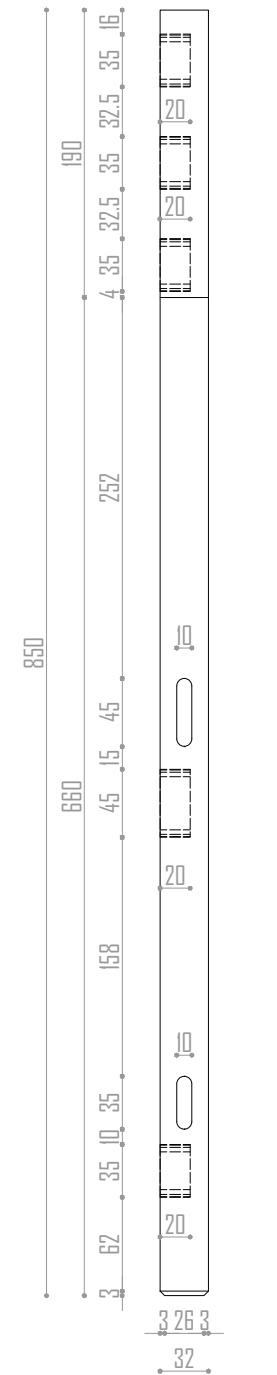
VISTA FRONTAL
