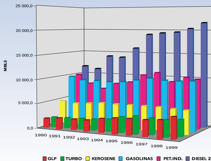
VENTAS INTERNAS DE DERIVADOS DE PETROLEO, POR TIPO DE PRODUCTO, 1990 - 1999 DOMESTIC SALES OF OIL BYPRODUCTS, BY TYPE OF PRODUCT, 1990 - 1999
